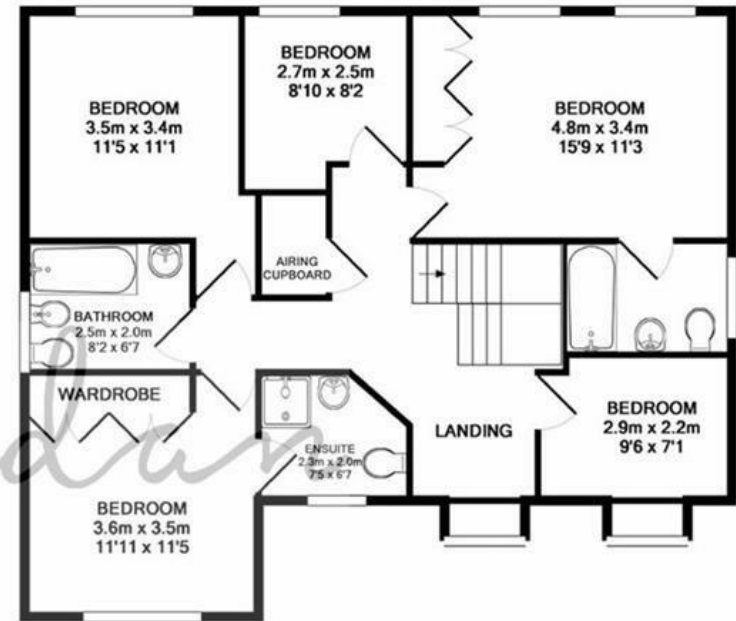
1ST FLOOR APPROX. FLOOR AREA 84.2 SQ.M. (907 SQ.FT.)
